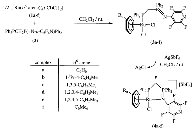
Scheme 1. Synthesis of ( \eta^6\text{-arene} )-ruthenium(II) complexes containing the iminophosphorane-phosphine ligand \text{Ph}_2\text{PCH}_2\text{P}(=\text{N-p-C}_5\text{F}_4\text{N})\text{Ph}_2 .
