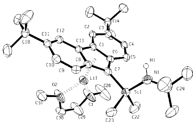
Figure 5. Molecular structure of [(3,6- t Bu 2 C 13 H 6 )SiMe 2 -NH + Bu]Li(DME) ( 5 ). Thermal ellipsoids are drawn at the 50% probability level; hydrogen atoms, except that on the N atom, are omitted for clarity. Selected bond distances (Å) and angles (deg): Li(1)–O(1), 1.939(5); Li(1)–O(2), 1.927(5); Li(1)–C(1), 2.342(5); Li(1)–C(6), 2.304(5); Li(1)–C(7), 2.291(5); Li(1)–C(8), 2.336(5); Li(1)–C(13), 2.375(5); Cent–Li, 1.982; N(1)–Si(1)–C(7), 107.15(12); Si(1)–C(7)–Li(1), 118.67(17); Cent–Li(1)–O(1), 139.73; Cent–Li(1)–O(2), 137.31 Cent is the centroid of C(1)–C(6)–C(7)–C(8)–C(13).
