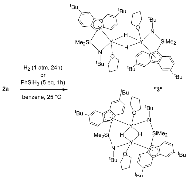
Scheme 1. Putative Dimeric Hydrido Structures for the Hydrogenolysis Product of 2a
