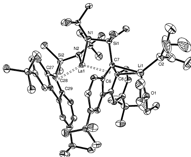
Figure 6. Molecular structure of 8 . Thermal ellipsoids are drawn at the 50% probability level; hydrogen atoms are omitted for clarity. Selected bond distances (Å) and angles (deg): La(1)–C(6), 3.025(4); La(1)–C(7), 2.806(4); La(1)–C(8), 2.883(4); La(1)–C(27), 2.843(4); La(1)–C(28), 2.766(4); La(1)–C(29), 3.068(4); Li(1)–C(7), 2.279(9); La(1)–N(1), 2.396(3); La(1)–N(2), 2.378(3); Li(1)–C(8), 2.439(9); Li(1)–O(1), 1.919(9); Li(1)–O(2), 1.910(9); N(1)–La(1)–N(2), 101.76(12); Cent(1)–La(1)–N(1), 75.86; Cent(2)–La(1)–N(2), 76.38; C(7)–Si(1)–N(1), 101.01(17); C(28)–Si(2)–N(2), 100.84(17). Cent(1) is the centroid of C(6)–C(7)–C(8); Cent(2) is the centroid of C(27)–C(28)–C(29).
