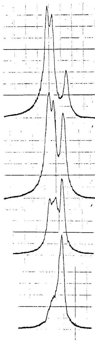
Figure 7. ^1\text{H} NMR of \text{C}_5\text{H}_5 resonances during reaction of 1 with \text{Cr}(\text{CO})_5\text{THF} . Top to bottom: 10%, 30%, 60%, and 90% complete reaction.
