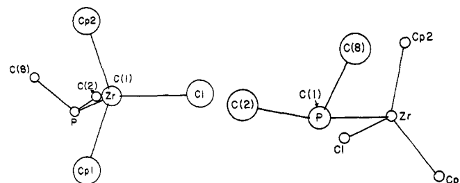
Figure 1. Newman projections sighting down Zr-C(1) (left) and P-C(1) bonds of \text{Cp}_2\text{Zr}(\text{Cl})\text{CH}_2\text{PPh}_2 (1).
