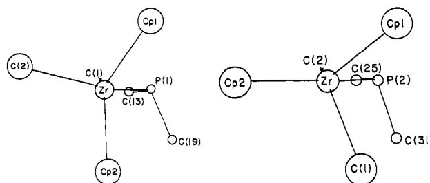
Figure 4. Newman projections sighting down Zr-C bonds of \text{Cp}_2\text{Zr}(\text{CH}_2\text{PPh}_2)_2 (4).
