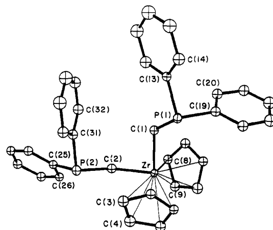
Figure 3. Representation of \text{Cp}_2\text{Zr}(\text{CH}_2\text{PPh}_2)_2 (4) with 50% thermal ellipsoids.
