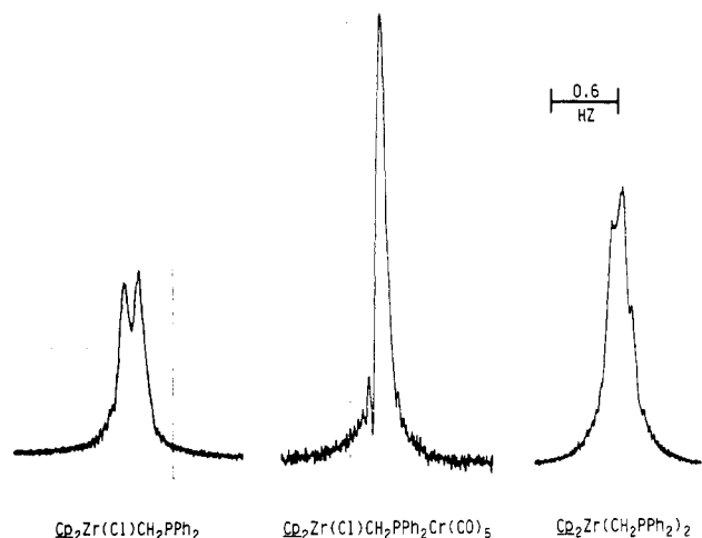
Figure 2. ^1\text{H} NMR \text{C}_6\text{H}_5 resonances for 1 (left), 12 (center), and 4 (right).
