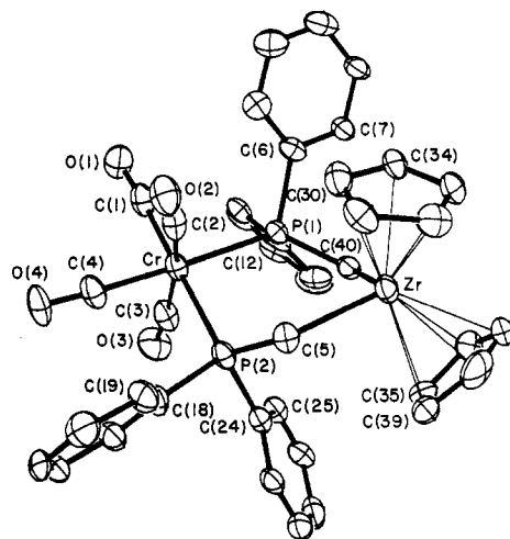
Figure 10. Representation of \text{Cp}_2\text{Zr}(\mu\text{-CH}_2\text{PPh}_2)_2\text{Cr}(\text{CO})_4 (17, \text{ML}_4 = \text{Cr}(\text{CO})_4 ).
