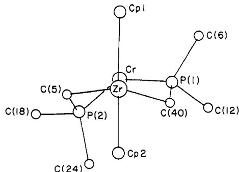
Figure 11. View of 17 ( ML_4 = Cr(CO)_4 ) looking approximately down Zr-Cr axis.
