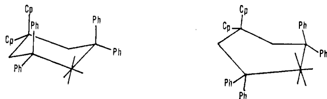
Figure 9. Sketches of chair (left) and twist-boat (right) conformations of \text{Cp}_2\text{Zr}(\mu\text{-CH}_2\text{PPh}_2)_2\text{ML}_4 (17).
