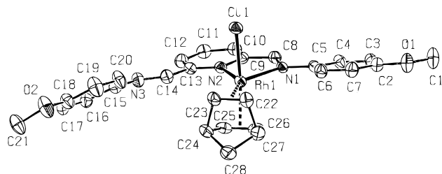
Figure 4. An ORTEP plot of complex 19 at 50% probability level along with the adopted numbering scheme. The hydrogen atoms and the cocrystallized molecule of dichloromethane have been left out for clarity.
