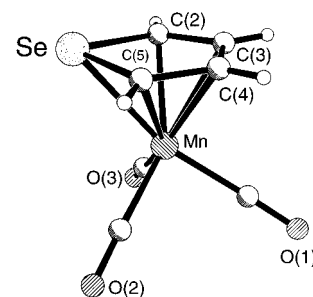
Figure 1. Crystal structure of the cation in [12]BF _4 . Selected bond lengths (Å) and angles (deg): Se–C(2) 1.877(4), Se–C(5) 1.883(4), Mn–Se 2.4298(6), Mn–C(2) 2.160(3), Mn–C(3) 2.161(3), Mn–C(4) 2.157(3), Mn–C(5) 2.159(3), O(1)–C(6)–Mn 178.3(3), O(2)–C(7)–Mn 177.8(3), O3–C(8)–Mn 176.6(4).
