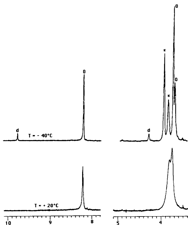
Fig. 1. Variable-temperature ^1\text{H} NMR spectra of [\{\text{Rh}(\text{NBD})\text{Cl}\}_2] : GCH = 1:1 mixtures in \text{CDCl}_3 ; *, [\{\text{Rh}(\text{NBD})\text{Cl}\}_2] ; 0, [\text{Rh}(\text{Cl})(\text{NBD})(\text{GCH})] ; d, [\{\text{Rh}_2(\text{NBD})_2\text{Cl}_2\}(\mu\text{-GCH})] .
