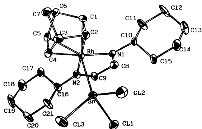
Fig. 2. View of [Rh(SnCl 3 )(C 7 H 8 )(C 14 N 2 H 24 )] showing the numbering scheme.
