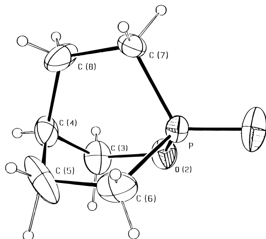
Figure 1. Molecular structure of 2 (PO 2 C 6 H 11 , fw 146.13, P 2 1 2 1 2 1 , colorless, a = 10.147(3) Å, b = 10.400(2) Å, c = 6.425(2) Å, Z = 4, R w = 0.0465, GOF = 1.68). Ellipsoids are drawn at the 50% probability level.
