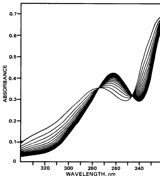
Figure 2 —UV spectral change associated with the alprazolam A = opened-ring-compound B reaction at pH 1.17 and room temperature; A + B = 4.02 \times 10^{-5} M; methanol, 10% (v/v); and repetitive scanning speed, 300 nm/min.
