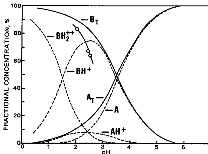
Figure 7—Fractional concentration of various ionic species involved in the \text{A} = \text{B} reaction as a function of pH. Open circles represent the total concentration of the opened-ring compound determined by a rapid back-titration technique.
