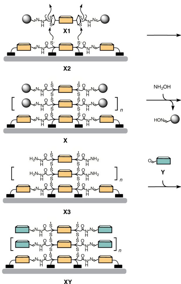
Figure 1. The SOSIP-TSE approach to double-channel surface architectures. Disulfide-exchange SOSIP yields the single-channel architecture X, TSE with chemo-orthogonal hydrazone exchange yields the double-channel architecture XY.
