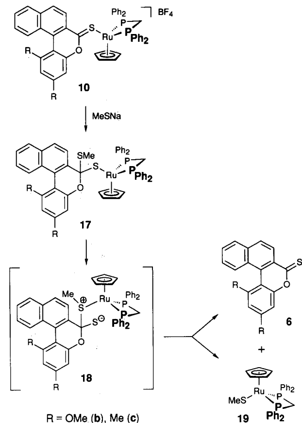
Scheme 8. Behavior of the dpdm complexes of type 10 towards S-nucleophiles.
