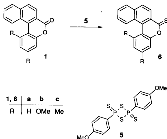
Scheme 2. Generation of the thionolactone 6 by oxygen/sulfur-exchange of 1 .
