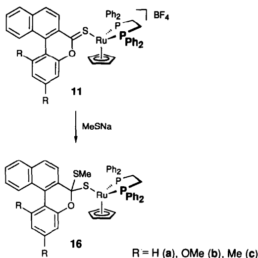
Scheme 7. Reaction of 11 with an S -nucleophile without subsequent cleavage of the \text{C}-\text{O} -bond.
