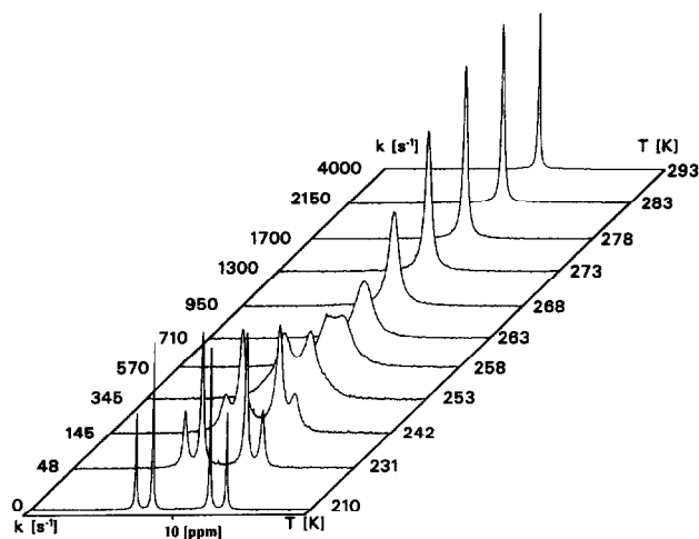
Fig. 2. Temperature-dependent ^{31}\text{P} NMR spectra of 10b .
