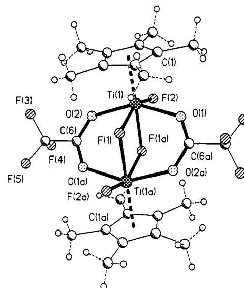
Figure 1. Molecular structure of (\text{Cp}^*\text{TiF}_2\text{OCOCF}_3)_2 ( 1 ).
