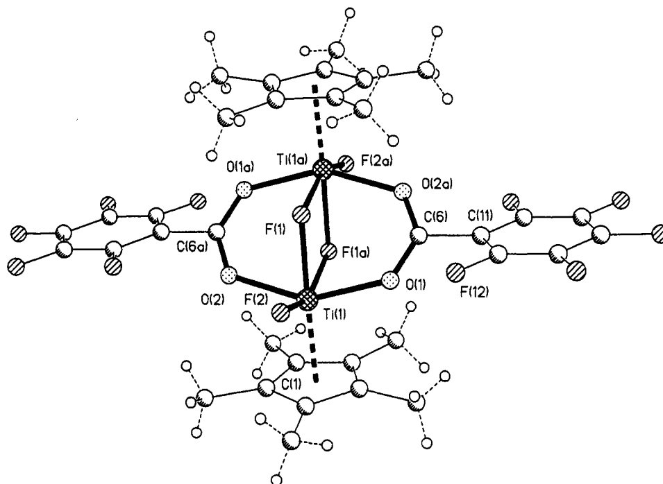
Figure 2. Molecular structure of (\text{Cp}^*\text{TiF}_2\text{OCOC}_6\text{F}_5)_2 ( 2 ).
