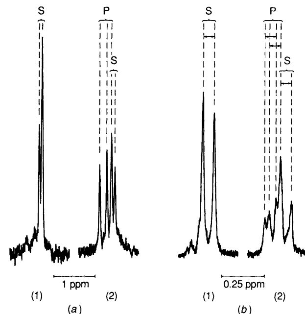
Figure 3. The ^1\text{H} NMR absorption of the methyl groups during the rearrangement in 99.7% trifluoromethanesulphonic acid of (a) 1,2,4-trimethyl-3-nitrobenzene (90 °C) and (b) 1,3-diisopropyl-2-nitrobenzene (54 °C). Spectrum (1) was taken near the start of reaction and spectrum (2) at about 60% reaction. S \equiv Starting material; P \equiv Product. In (b), the double-headed arrows connect the two signals of a given isopropyl group.
