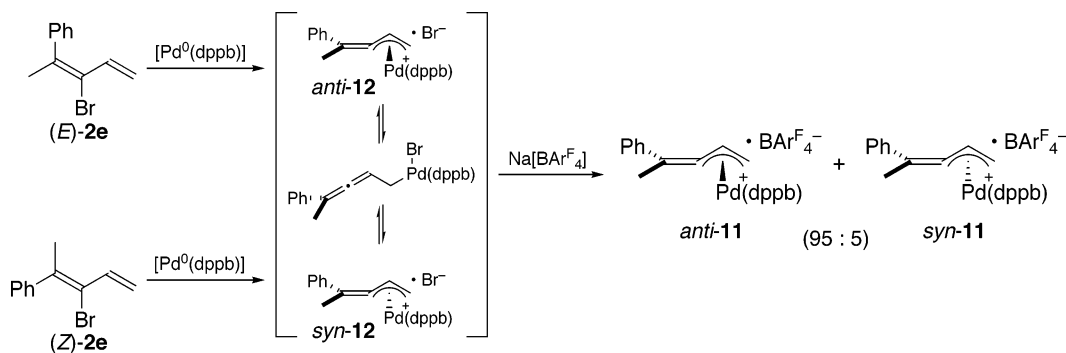
Scheme 7
