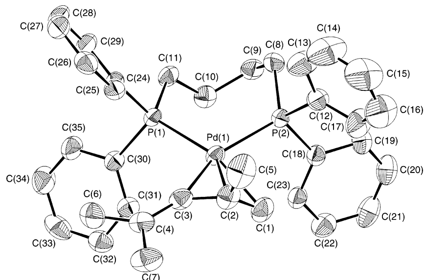
Figure 1. ORTEP drawing of the cation in [\text{Pd}(\eta^3\text{-CH}_2\text{CMeC=Me}_2)(\text{dppb})]\text{BARF}_4 ( 1 ) with 30% thermal ellipsoids. The \text{BARF}_4^- anion and all hydrogen atoms are omitted for clarity.
