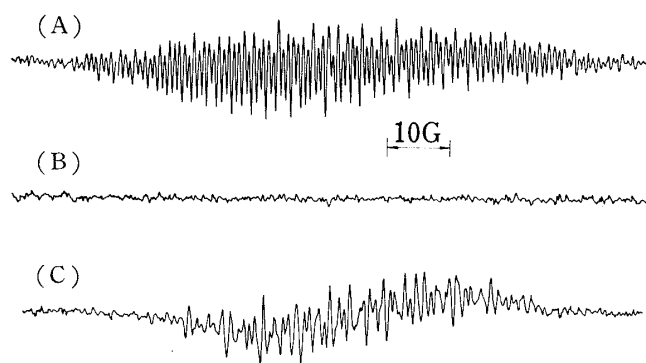
Fig. 1. ESR Spectra of the Aminopyrine Free Radical (A) and the 4-Diethylaminoantipyrene Free Radical (C)
