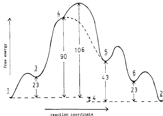
Figure 4. Reaction profile for 1a \rightleftharpoons 2a . The free energies given are kJ mol -1 .
