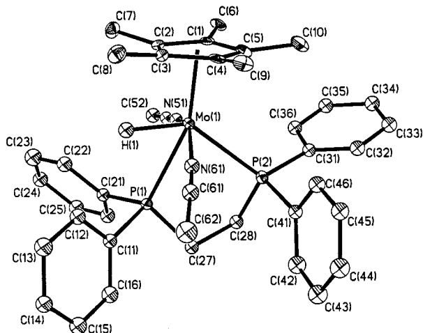
Figure 2. A view of the [\text{Cp}^*\text{MoH}(\text{MeCN})_2(\text{dppe})]^+ cation for compound 2 . Carbon-bonded hydrogen atoms are omitted for clarity. Selected bonding parameters (CNT = Cp* center of gravity): Mo–CNT, 1.998(7) Å; Mo–P1, 2.541(2) Å; Mo–P2, 2.554(2) Å; Mo–H1, 1.69(6) Å; Mo–N51, 2.137(6) Å; Mo–N61, 2.122(6) Å; CNT–Mo–H1, 100(2)°; CNT–Mo–N51, 103.1(2)°; CNT–Mo–N61, 104.8(2)°; CNT–Mo–P1, 159.5(2)°; CNT–Mo–P2, 121.6(2)°.
