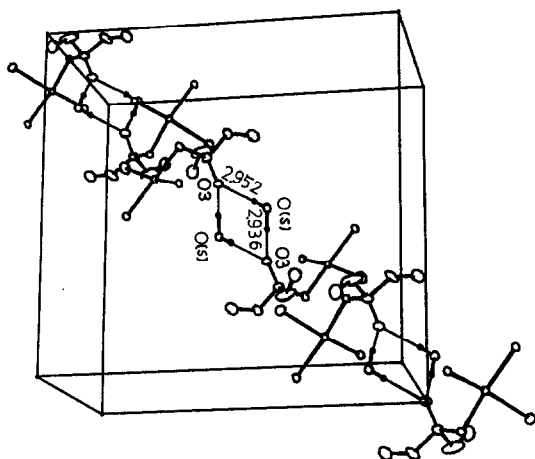
Fig. 3. Hydrogen bonding between solvent \text{H}_2\text{O} molecule and phosphonate oxygen atoms in cis - \text{Pt}(\text{PPh}_3)_2(\text{I})(\text{CH}_2\text{P}(\text{O})(\text{OCH}_3)_2) \cdot \text{H}_2\text{O} .
