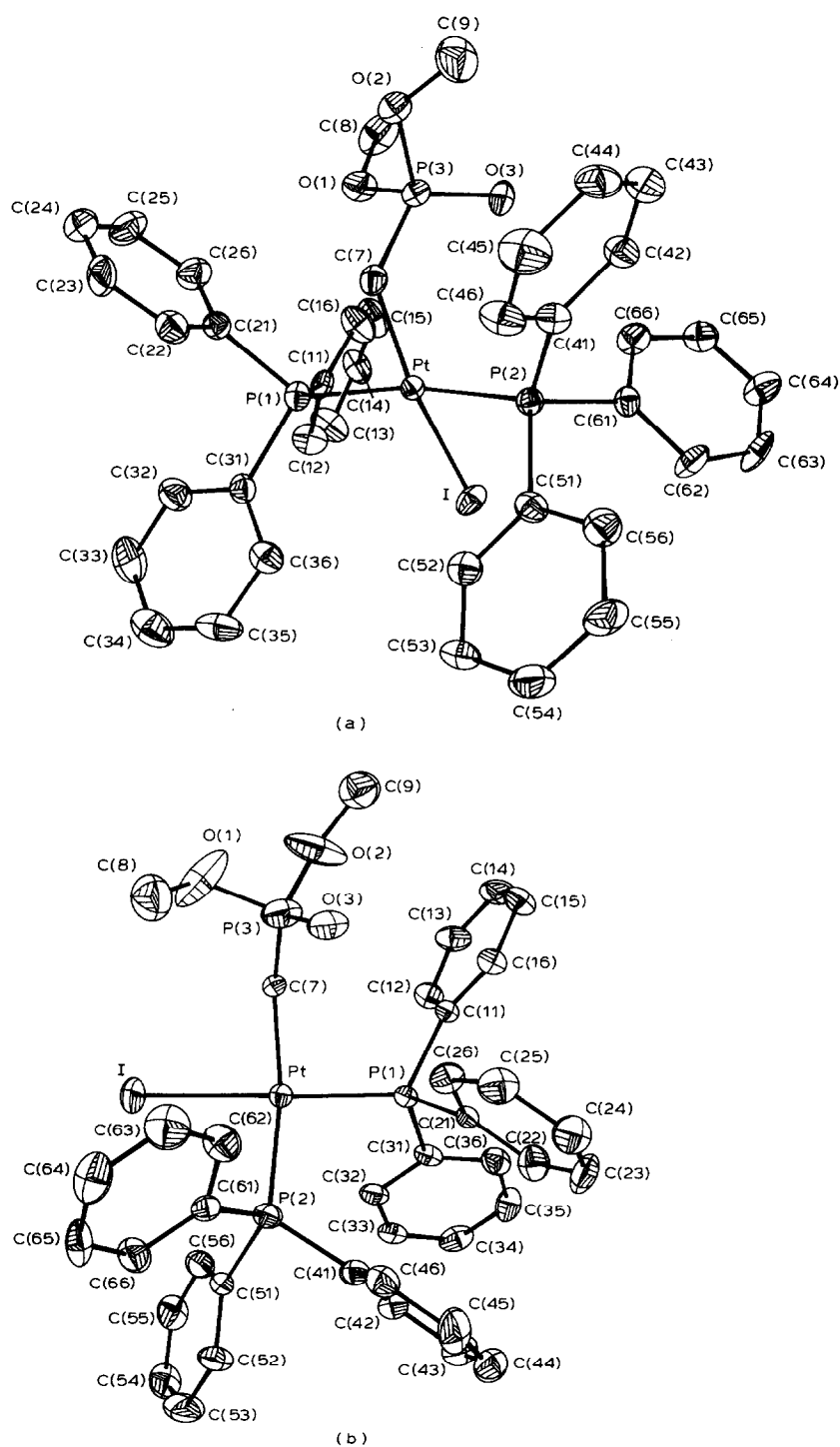
Fig. 2. Molecular structures of \text{Pt}(\text{PPh}_3)_2(\text{I})(\text{CH}_2\text{P}(\text{O})(\text{OCH}_3)_2)_2 ; (a) trans ; (b) cis .
