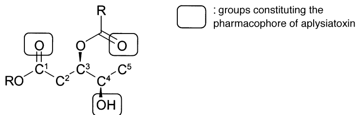
Fig. 5. (3 R ,4 R )-Dihydroxypentanoyl unit comprising the pharmacophores of aplysiatoxin
