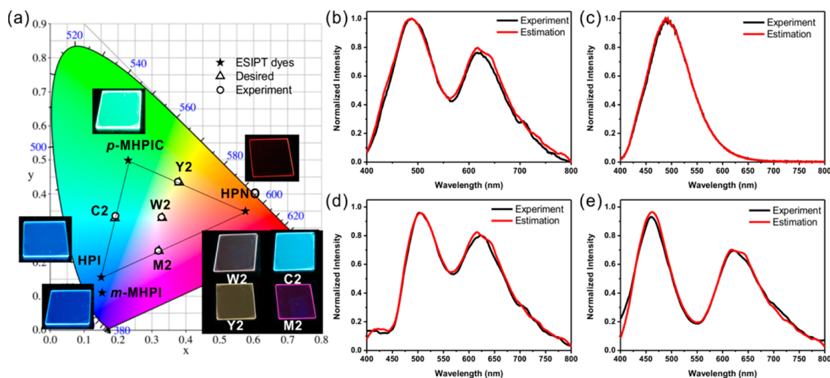
Figure 4. (a) Emission color coordinates of the ESIPT dye-doped PMMA film mixtures (total c = 1 wt %) in the CIE 1931 chromaticity diagram: individual ESIPT dyes ( \star , m -MHPI, HPI, p -MHPIC, and HPNO), desired values ( \Delta ), and experimentally obtained values of the mixtures ( \circ , W2, C2, Y2, and M2). The inset shows the photographs of the individual ESIPT dyes and the corresponding mixtures under 340 nm UV light. Normalized emission spectra of the corresponding film mixtures: (b) W2, (c) C2, (d) Y2, (e) M2. The excitation wavelength was 340 nm.
