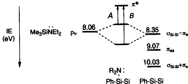
Fig. 1. Qualitative MO model for the origin of two absorptions of (amino)(phenyl)disilanes.
