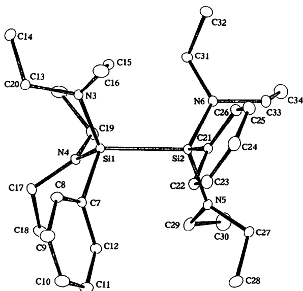
Fig. 3. Crystal structure of 3 . Hydrogen atoms are omitted for clarity.
