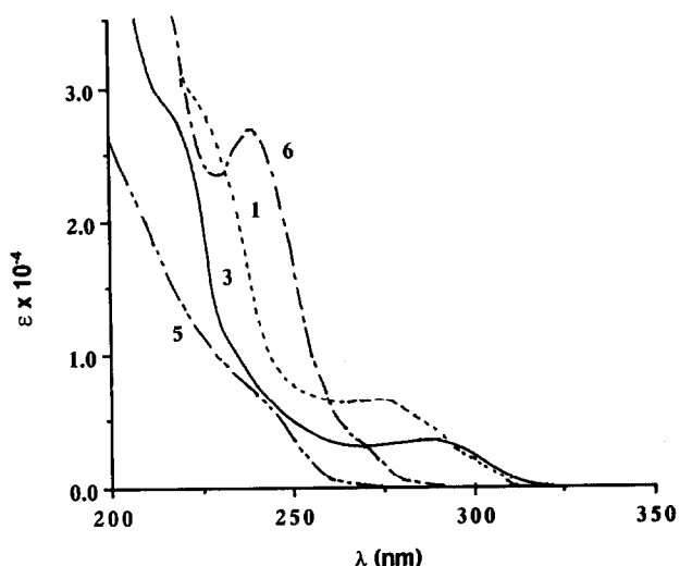
Fig. 2. UV spectra of 1, 3, 5 and 6 in cyclohexane.
