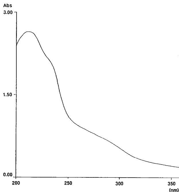
Fig. 4. UV spectrum of 3 in the solid state (KBr pellet).
