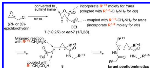
Scheme 1. General Synthetic Scheme for the Designed Mimetics
