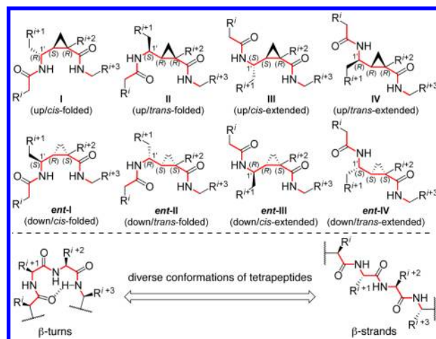
Figure 2. Designed tetrapeptide-mimetic scaffolds.
