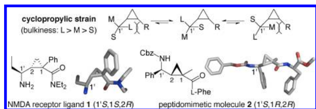
Figure 1. Diagram of the cyclopropyl strain, and the X-ray crystal structures of 1 and 2 .
