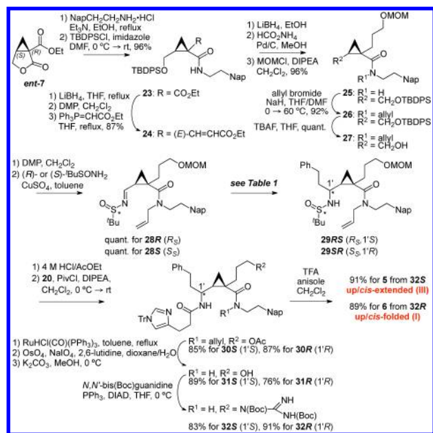
Scheme 3. Synthesis of cis -type Mimetics 5 and 6
