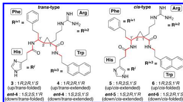
Figure 3. Designed MCR ligands.
