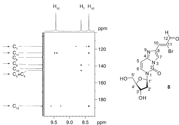
Figure 1. ^1\text{H} - ^{13}\text{C} HMBC of 8 in \text{DMSO}-d_6 at 600 MHz.
