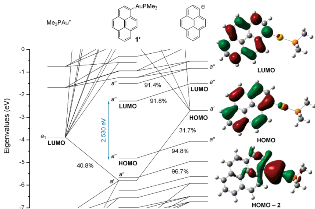
Figure 3. (left) Kohn–Sham orbital energy-level diagram of (\text{Me}_3\text{P})\text{Au}(1\text{-pyrenyl}) ( \mathbf{1}' ) (mpw91/ Stuttgart ECP and basis on Au). Implicit THF solvation is included through a polarizable continuum model. Percentage contributions of (phosphine)gold(I) cation and pyrenyl anion fragments are indicated. (right) Plots of selected orbitals (contour level 0.03 au).
