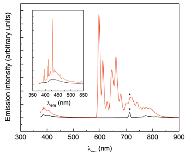
Figure 2. Emission spectra (77 K, red; 298 K, black; 355 nm excitation) of (\text{Cy}_3\text{P})\text{Au}(1\text{-pyrenyl}) ( 1 ; 5 \times 10^{-6} \text{ M} ) in degassed 2-MeTHF. Inset: emission of 1 at 5 \times 10^{-8} \text{ M} under otherwise identical conditions. No luminescence is observed past 550 nm at this concentration. Note that y axes of the two spectra have different scales. An asterisk indicates the excitation pulse second harmonic.
