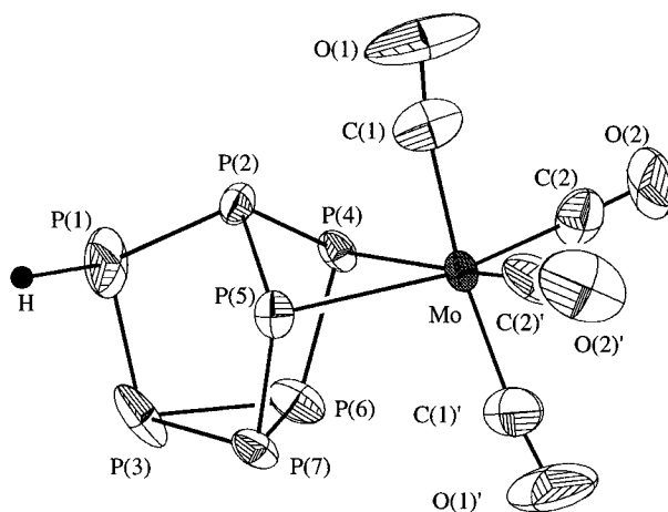
Figure 1. ORTEP drawing of the [\eta^2\text{-HP}_7\text{Mo}(\text{CO})_4]^{2-} ion ( 5b ). The H atom was placed in an idealized position and was not located crystallographically.
