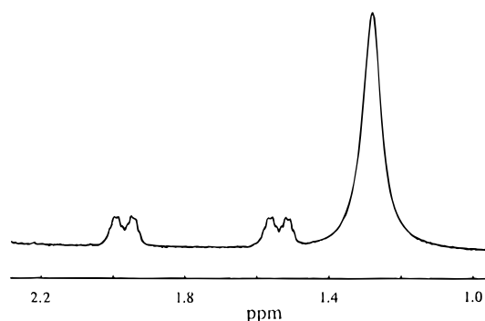
Figure 5. ^1\text{H} NMR spectrum for the [\eta^2\text{-HP}_7\text{W(CO)}_4]^{2-} ion ( 5a ) recorded at 27 °C and 400 MHz from \text{dmf-}d_7 solution. The singlet at 1.3 ppm is associated with the en solvate molecule.
