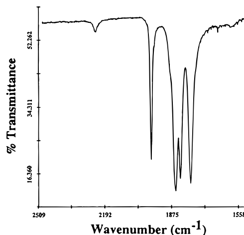
Figure 6. Solid-state IR spectrum (KBr pellet) showing the P–H and carbonyl regions of the [\eta^2\text{-HP}_7\text{Mo(CO)}_4]^{2-} ion ( 5b ).
