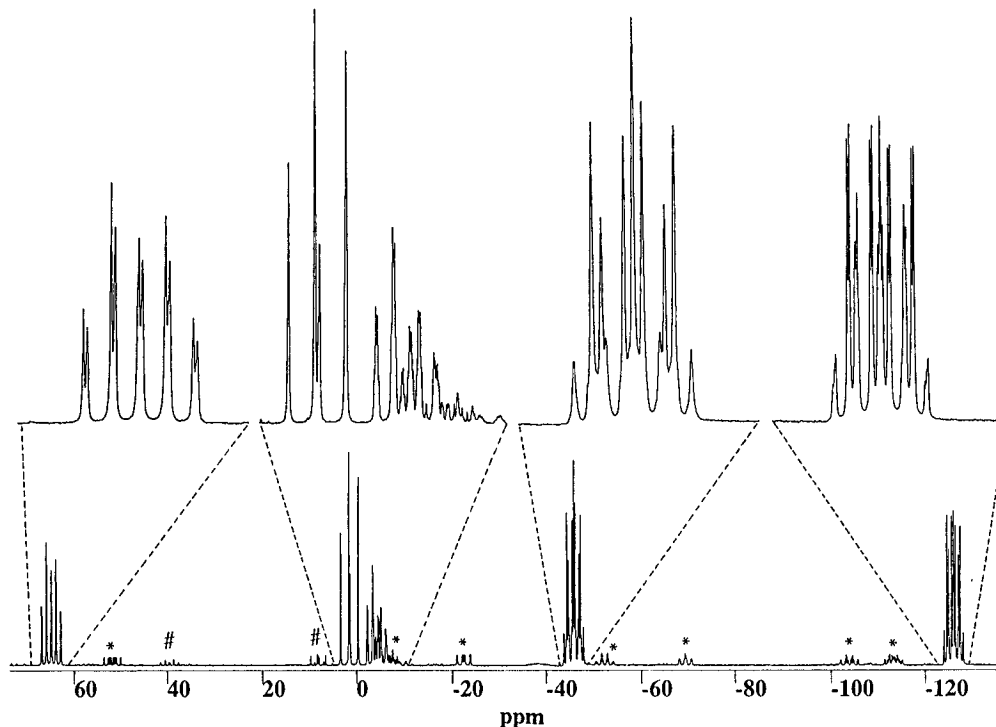
Figure 3. ^{31}\text{P} NMR spectrum of [\eta^2\text{-P}_7\text{W(CO)}_4]^{3-} ( 4a ) recorded at 25 °C and 202 MHz in \text{dmf-}d_7 solution. The resonances marked with (*) arise from [\eta^2\text{-HP}_7\text{W(CO)}_4]^{2-} impurities. The resonances marked with (#) arise from an unidentified impurity.
