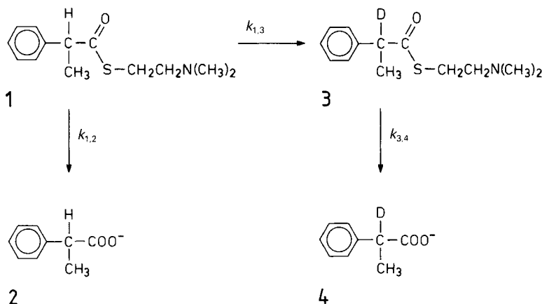
Scheme 2. Chemical Reactions of Hydrolysis and ^1\text{H}/^2\text{H} Exchange Observed in the Investigated Deuterated Solvent/ \text{D}_2\text{O} Mixtures. The compounds are: S -[(dimethylamino)ethyl] 2-phenylpropanethioate (1); S -[2-(dimethylamino)ethyl] 2-phenyl[2- ^2\text{H}_1 ]propanethioate (3); 2-phenylpropionic acid (2); 2-phenyl[2- ^2\text{H}_1 ]propionic acid (4).
