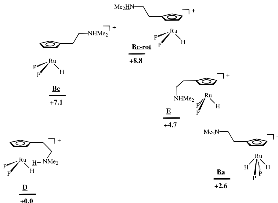
Figure 9. Proposed mechanism for the intramolecular exchange of the two hydrogen atoms involved in the dihydrogen bond (relative energies in \text{kcal}\cdot\text{mol}^{-1} ).
