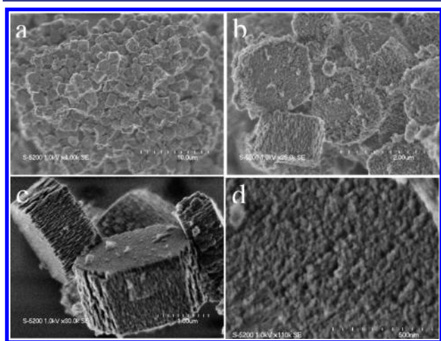
Figure 1. (a) Low- and (b–d) high-magnification SEM images of a calcined ZSM-5 sample synthesized in the presence of C-PSt- co -P4VP template showing oriented mesopores.
