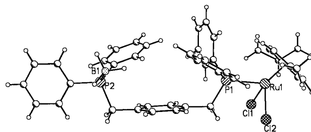
Figure 3. Alternative view illustrating the syn-orientation of the P atoms of 3 .
