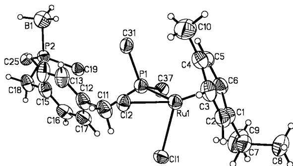
Figure 2. Projection of the structure of [(p\text{-cym})\text{RuCl}_2\text{PPh}_2\text{CH}_2\text{C}_6\text{H}_4\text{CH}_2\text{Ph}_2\text{P-BH}_3] , 3 , with 50% thermal ellipsoids.
