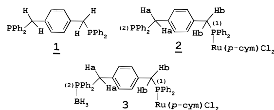
Figure 1. Diagrammatic representation of compounds 1 – 3 .
