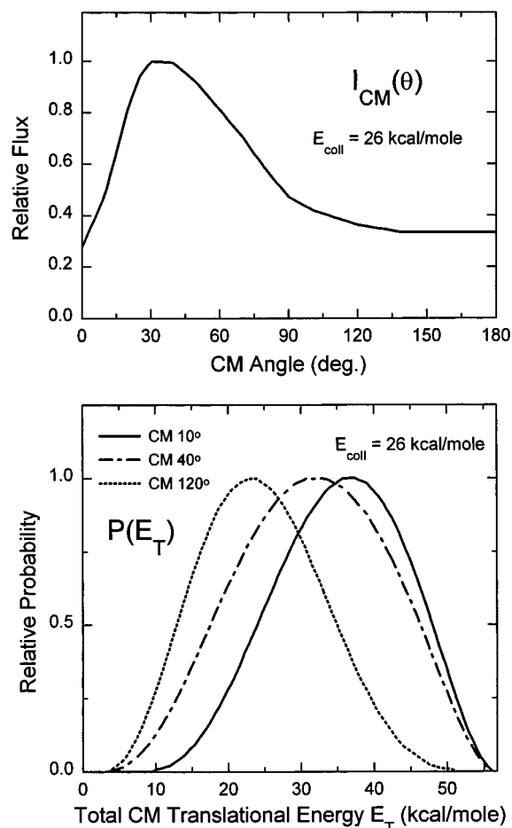
Figure 4. Upper: total CM angular distribution I_{\text{CM}}(\theta) at E_{\text{coll}} = 26 kcal/mol. The maximum of the relative angular distribution is scaled to unit. Lower: total CM product translational energy distribution P(E_T) at various CM angles at E_{\text{coll}} = 26 kcal/mol. Maximum probabilities are scaled to unit. The maximum translational energy is the total available energy at the most probable collision energy E_{\text{coll}} = 26 kcal/mol.
