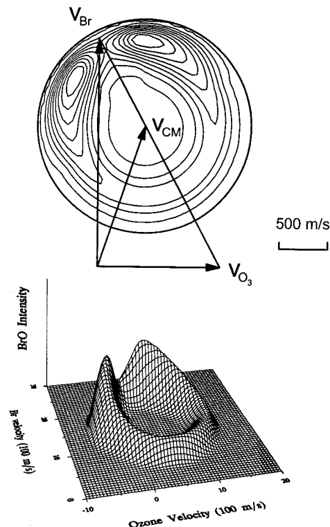
Figure 5. Contour map and the 3-D plot for the CM flux-velocity distribution I_{\text{CM}}(\theta, u) at E_{\text{coll}} = 26 kcal/mol.
