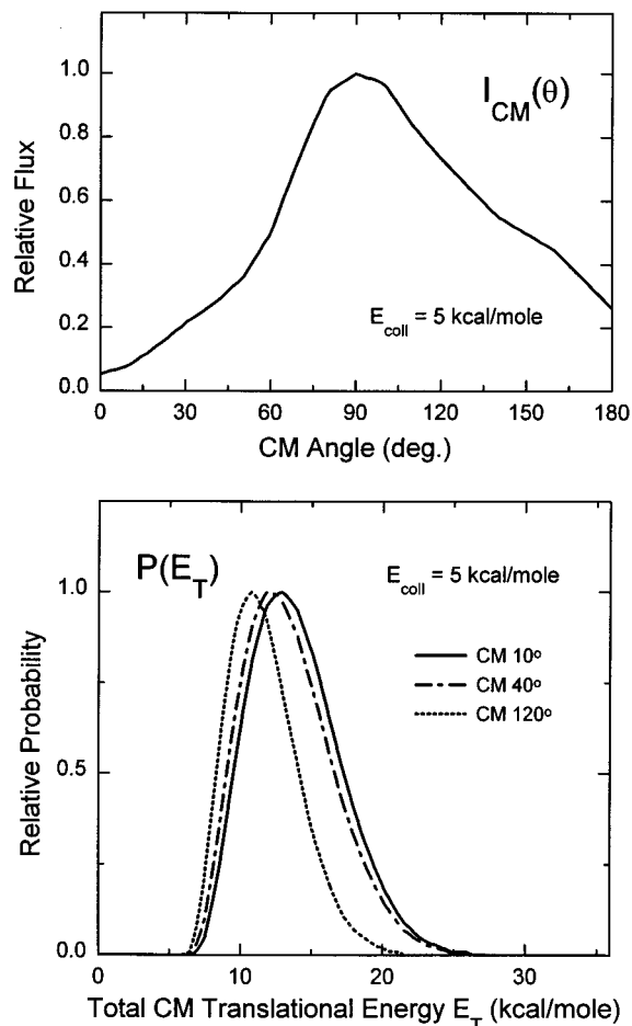
Figure 14. Same as Figure 4 but at E_{\text{coll}} = 5 kcal/mol.
