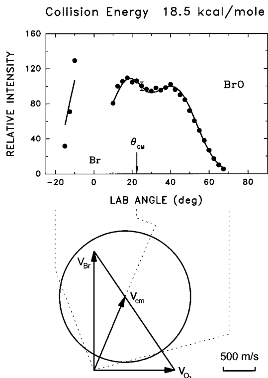
Figure 6. Same as Figure 2 but at E_{\text{coll}} = 18.5 kcal/mol.
