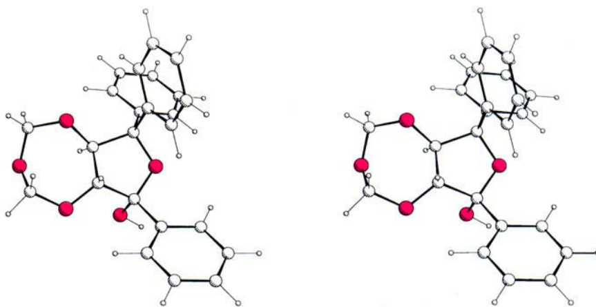
Fig. 1. Stereo PLUTO presentation of 8 in the solid state. Only one of the two H-brided molecules in the asymmetric unit is depicted.
