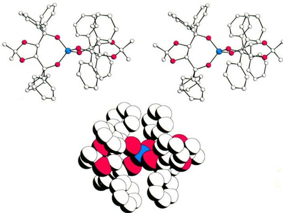
Fig. 9. Stereo PLUTO presentation and a space-filling presentation of one of the three spiro-titanate molecules in the crystal structure of [3 \cdot 10 \cdot 0.5 \text{ Et}_2\text{O}] . The H-atoms have been omitted for clarity.
