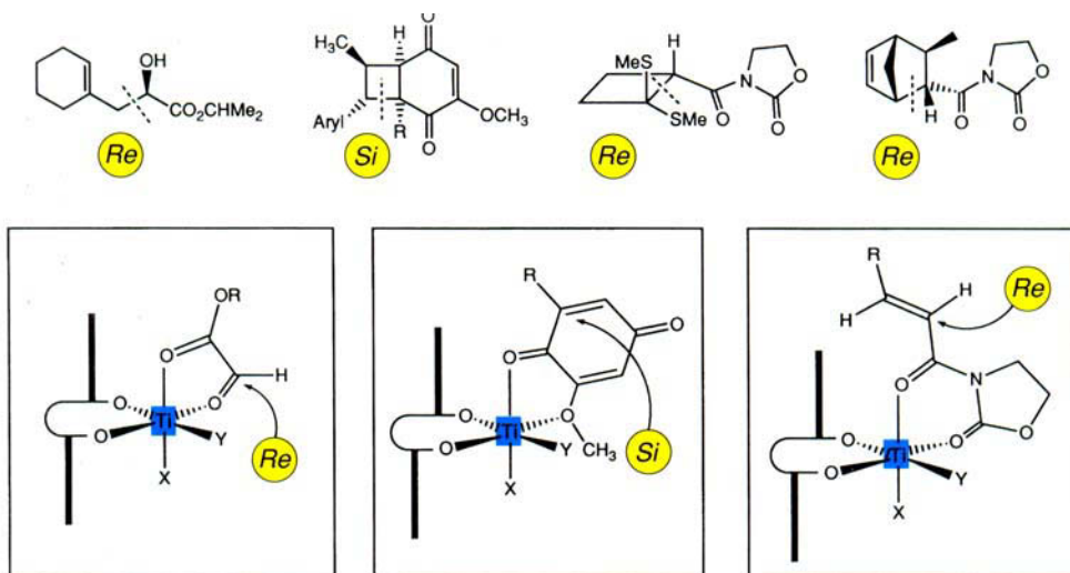
Fig. 12. Products of an ene reaction and of [2 + 2] and [4 + 2] cycloadditions mediated or catalyzed by a complex of type 11 and the corresponding models for the Ti complexes of the bidentate electrophiles used. Top, left to right: major product (72:28) from methylidenecyclohexane and isopropyl glyoxylate [23], cyclobutane derivative (ca. 95:5) from methylstyrene and methoxy-quinones [68], thioacetal of a cyclobutanonecarboxylic-acid derivative (94:6) from 3-acryloyl-1,3-oxazolidin-2-one and a ketene dithioacetal [69], and a norbornenecarboxylic-acid derivative (> 95:5) obtained by Diels-Alder reactions with the corresponding N -crotonoylheterocycle [15] [16] [20]. Bottom: binding of the bidentate electrophiles, used for the above reactions, on a Ti with octahedral ligand sphere (X, Y represent additional ligands) such that the observed products would result by approach of nucleophiles in an octand not facing a quasi axial Ph group. The picture would be similar with a trigonal bipyramidal ligand sphere around Ti, see comments in the caption of Fig. 11. For discussions and mechanistic proposals concerning the Diels-Alder addition, see also [15] [24b].
