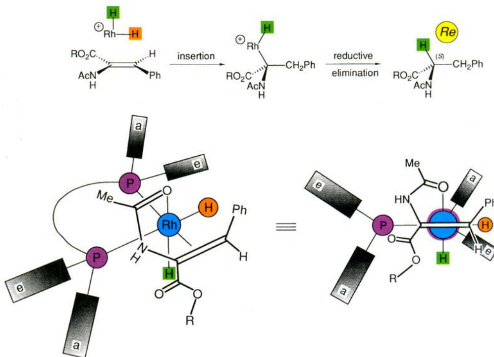
Fig. 13. Hydrogen transfer to C(2) of aminocinnamates from the Re -face in catalytic hydrogenations by Rh complexes of C 2 -symmetrical diphosphines. The Rh complexes of ( S,S )-DIOP, ( M )-BINAP, ( R,R )-CHIRAPHOS, ( R,R )-DIPAMP, and ( R,R )-BMPPP all lead to ( S )-phenylalanine derivatives. For the structures of corresponding phosphine complexes, see bottom part of Table 7. The substrate is complexed in such a way that a) the N -acetyl ligand is located near the quasiequatorial substituent on the P-atom, b) the Ph group of the cinnamate resides in an unhindered position, c) the C=C bond inserts into the Rh–H bond which is ' trans ' to one of the P-atoms, and d) insertion occurs with a coplanar arrangement of the two double-bond C-atoms, the Rh- and the H-atoms. Except for the sense of chirality and the specification of the position of the substituents on the P-atoms, the general complex shown here is identical to the intermediate proposed by Halpern et al. (3 min in Fig. 2 and 9 of [64]). Unfortunately, in the same paper and in many other related publications, there are alternative presentations (with the H-atoms trans to the NCOMe ligand being transferred first, or with a perpendicular arrangement of the C=C bond with respect to the Rh–H bond prior to insertion!).
