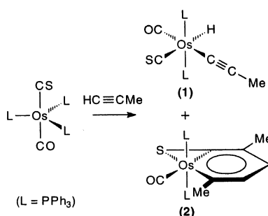
Scheme 1. Synthesis of the new 3,6-dimethyl-substituted osmabenzene, \text{Os}(\eta^2\text{-C[S]CMeCHCHCMe})\text{(CO)(PPh}_3)_2 ( 2 ).
