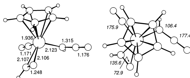
Fig. 6. DFT optimised geometry of [(C_5H_5)(CO)W(NCH)(HC=C=O)] , in a side view (left) and a top view (right). Bond distances (Å) are given in normal typeface, angles (°) in italics .
