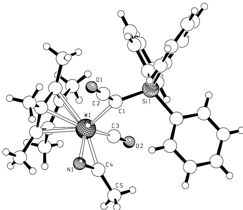
Fig. 3. Molecular structure of [(\text{C}_5\text{Me}_5)(\text{CO})(\text{NCMe})\text{W}\{\text{C}(\text{SiPh}_3)=\text{C}=\text{O}\}] ( 8 ). Important distances ( \text{\AA} ) and angles ( ^\circ ) with estimated S.D. in parentheses: W1-C1 2.174(3), W1-C3 1.942(4), W1-C4 2.058(4), W1-N1 2.020(3), W1-C(\text{C}_5\text{Me}_5) 2.295(4)–2.446(4), C1-C2 1.296(5), C1-\text{Si1} 1.848(4), C2-O1 1.180(5), C3-O2 1.165(5), C4-N1 1.257(5), C4-C5 1.487(5); C2-C1-\text{Si1} 123.4(3) , W1-C1-C2 105.2(3) , W1-C1-\text{Si1} 123.4(3) , C1-C2-O1 178.5(4) , W1-C3-O2 174.7(3) , N1-C4-C5 136.1(4) .
