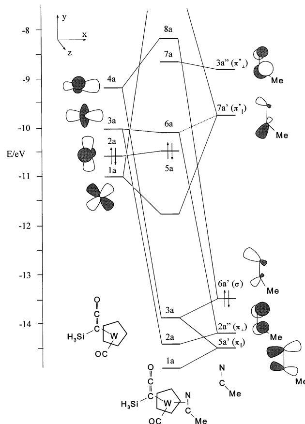
Fig. 5. Molecular orbital diagram for the interaction between [(C_5H_5)(CO)W\{C(SiH_3)=C=O\}] and NCMe.
