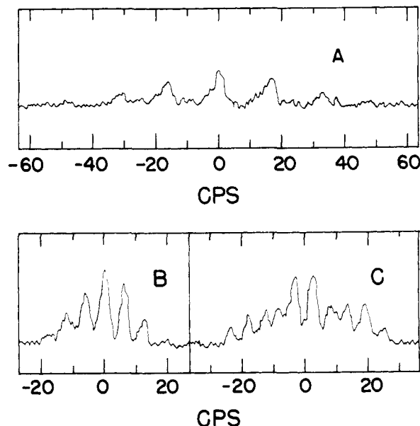
Fig. 1.—The high resolution fluorine magnetic resonance absorption spectrum of (\text{CF}_3)_2\text{NCF}_2\text{CF}_3 , observed at a fixed frequency of 16.685 Mc. A, B and C are the absorption of the \text{N}-\text{CF}_2 -, \text{C}-\text{CF}_3 and (\text{CF}_3)_2\text{N} groups, centered at \delta values of -1.99, -0.85 and +2.31, respectively.
