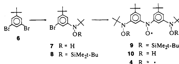
Scheme I. Synthetic Route to Trinitroxide 4
