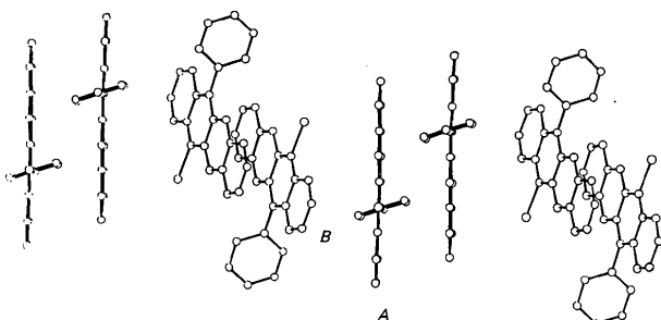
Fig. 4. Extended view of the crystal lattice of 5-bromo-12-phenyltetracene with the two molecules A and B in the asymmetric unit labelled.
