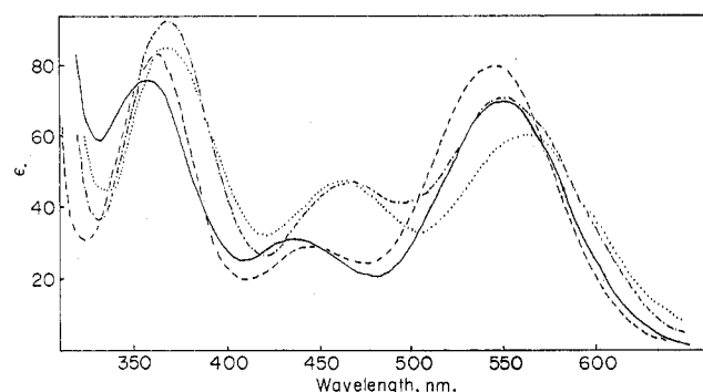
Figure 1.—Electronic absorption spectra: trans -[Co(2,3,2-tet)(glyH) 2 ](ClO 4 ) 3 , —; trans -[Co(2,3,2-tet)(OAc) 2 ](ClO 4 ) 3 , ----; trans -[Co(3,2,3-tet)(glyH) 2 ](ClO 4 ) 3 , .....; trans -[Co(3,2,3-tet)(OAc) 2 ](ClO 4 ) 3 , -.-.-.-.-.
