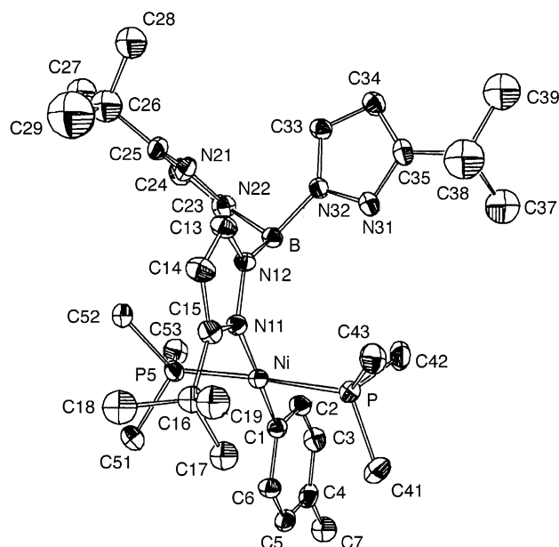
Fig. 2. The molecular structure of compound 5b .
