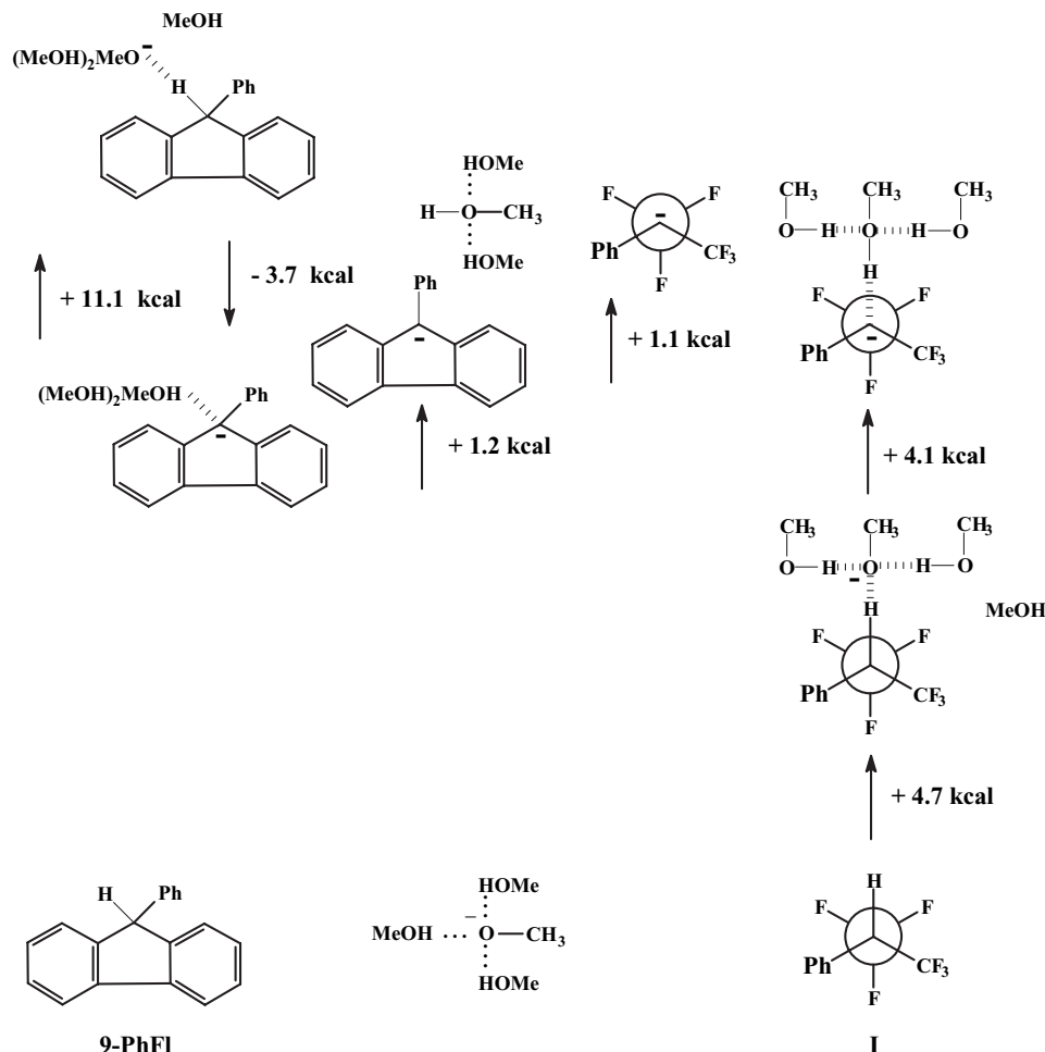
Figure 4. Energies calculated using B3LYP/6-31+G(d,p) for 9-PhFI and I
