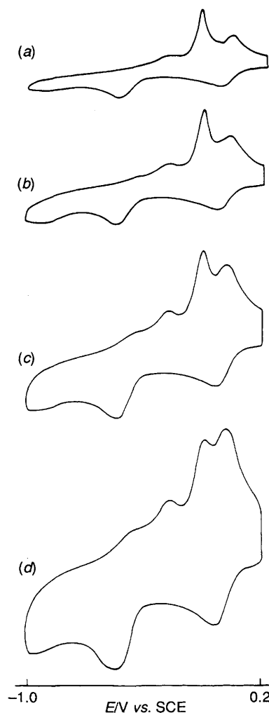
Fig. 7 Cyclic voltammograms of complex 2 recorded in MeCN solution, 0.2 \text{ mol dm}^{-3} in \text{K}[\text{PF}_6] , recorded at scan rates of (a) 100, (b) 200, (c) 500 and (d) 1000 \text{ mV s}^{-1}
