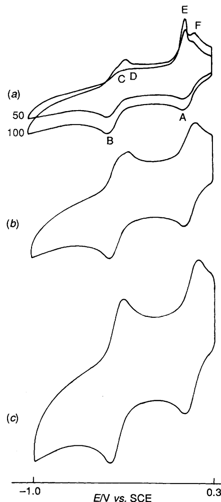
Fig. 6 Cyclic voltammograms of complex 2 recorded in MeCN solution, 0.2 \text{ mol dm}^{-3} in \text{Na}[\text{ClO}_4] , recorded at scan rates of (a) 50 and 100, (b) 200 and (c) 500 \text{ mV s}^{-1}
