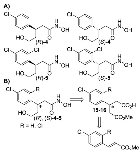
Scheme 1. (A) Structures of Hydroxamates ( R )- and ( S )- 4 and -5 ; (B) Retrosynthetic Analysis
