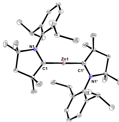
Figure 1. Molecular structure of 2. H atoms are omitted for clarity. Anisotropic displacement parameters are depicted at the 50% probability level. Selected experimental [calculated at RI-BP86/def2-SVP singlet; triplet; singlet biradical] bond lengths [ \text{\AA} ] and angles [ ^\circ ]: \text{Zn1}\text{--}\text{C1} 1.8850(17) [ 1.896 ; 1.924 ; 1.902 ], \text{C1}\text{--}\text{N1} 1.376(2) [ 1.388 ; 1.398 ; 1.392 ], \text{C1}\text{--}\text{C1}' 3.770 [ 3.791 ; 3.851 ; 3.805 ], \text{C1}\text{--}\text{Zn1}\text{--}\text{C1}' 180.0 [ 180.0 ; 177.6 ; 180.0 ].
