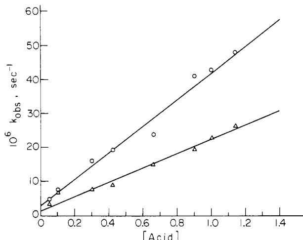
Figure 1. Observed rate constant for hydrolysis of 1 (O) and 2 (Δ) as described in the text.
