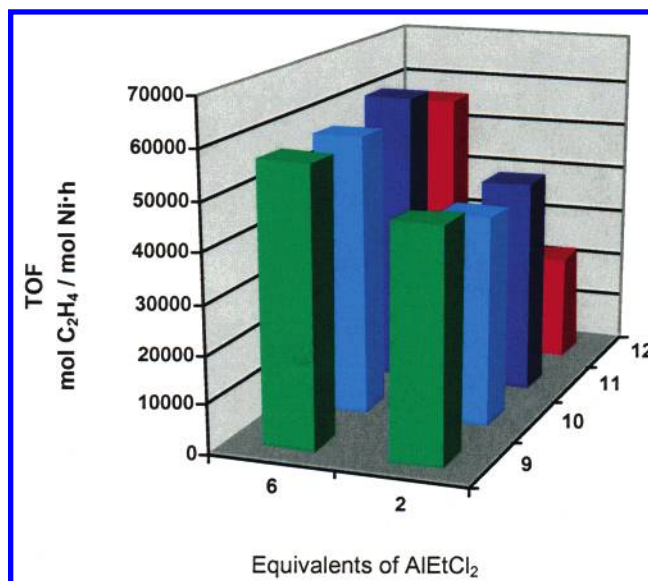
Figure 1. Activity of complexes 9–12 for the oligomerization of ethylene using different quantities of AlEtCl 2 . Conditions: T = 30\text{ }^{\circ}\text{C} , 10 bar of C 2 H 4 , 35 min, 4 \times 10^{-2} mmol of Ni, 15 mL of toluene.
