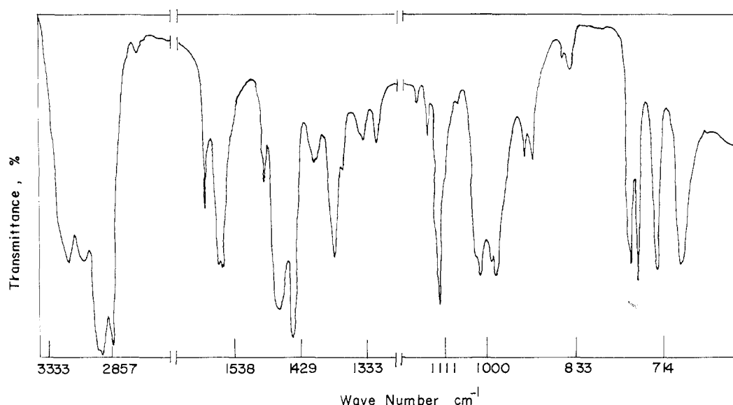
Figure 1.—Infrared spectrum of [(\text{C}_6\text{H}_5)_2\text{P}(\text{NH}_2)_2]\text{Cl} (Nujol).
