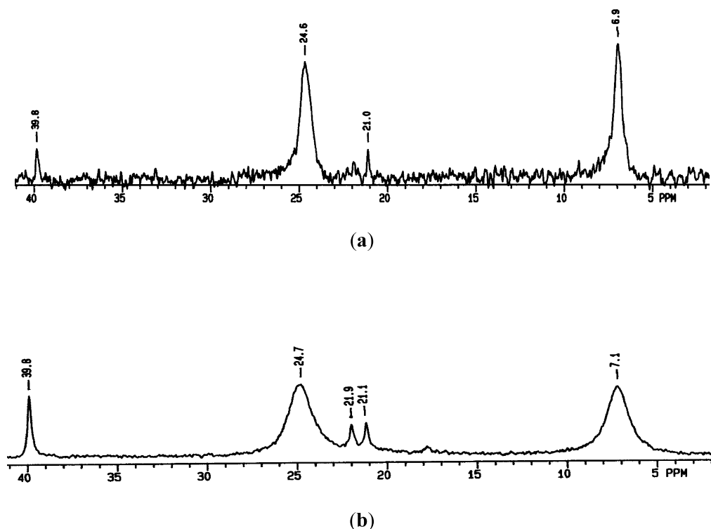
Fig. 2. ^{31}\text{P} -NMR spectrum of: (a) freshly prepared \text{Ph}_3\text{Sn}[(\text{OPMe}_2)(\text{OPPh}_2)\text{N}] ; and (b) 6-h old \text{Ph}_3\text{Sn}[(\text{OPMe}_2)(\text{OPPh}_2)\text{N}] .
