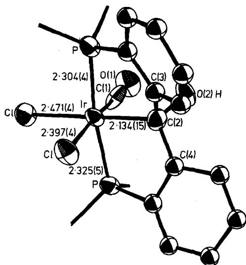
Fig. 2. Molecular structure of \text{IrCl}_2(\text{o-PPh}_2\text{C}_6\text{H}_4\text{C[OH]C}_6\text{H}_4\text{PPh}_2\text{-o})(\text{CO}) with phenyl rings omitted for clarity. Important bond angles are: \text{P-Ir-P} 167.9(1), \text{Ir-C(2)-O(2)} 109.9(9), \text{Ir-C(2)-C(3)} 112(1), \text{Ir-C(2)-C(4)} 107(1), \text{C(3)-C(2)-O(2)} 109(1), \text{C(4)-C(2)-O(2)} 108(1), \text{C(3)-C(2)-C(4)} 115(1)°.
