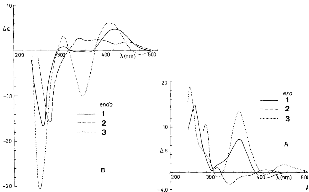
Fig. 4. CD spectra of (A) exo - and (B) endo -complexes 1 – 3
