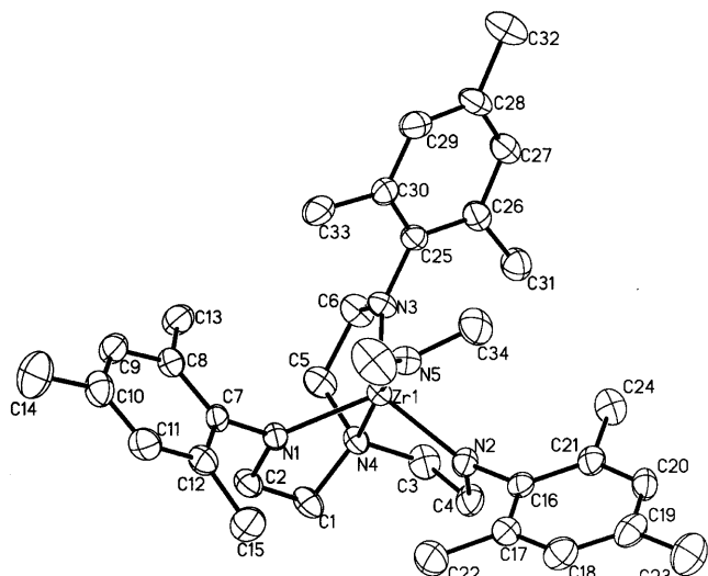
Fig. 1. Thermal ellipsoid plot of the molecular structure of [\text{Zr}(\text{TMT})(\text{NMe}_2)] ( 5 ) (non-hydrogen atoms). Selected distances (Å) and angles (°): \text{Zr}(1)-\text{N}(3) 2.108(3), \text{Zr}(1)-\text{N}(1) 2.119(3), \text{Zr}(1)-\text{N}(2) 2.124(3), \text{Zr}(1)-\text{N}(5) 2.044(3), \text{Zr}(1)-\text{N}(4) 2.393(3), \text{N}(3)-\text{Zr}(1)-\text{N}(2) 109.42(13), \text{N}(3)-\text{Zr}(1)-\text{N}(1) 109.53(13), \text{N}(2)-\text{Zr}(1)-\text{N}(1) 118.23(13), \text{N}(3)-\text{Zr}(1)-\text{N}(5) 108.78(13), \text{N}(2)-\text{Zr}(1)-\text{N}(5) 101.23(13), \text{N}(1)-\text{Zr}(1)-\text{N}(5) 109.09(13), \text{N}(3)-\text{Zr}(1)-\text{N}(4) 74.81(12), \text{N}(2)-\text{Zr}(1)-\text{N}(4) 73.64(12), \text{N}(1)-\text{Zr}(1)-\text{N}(4) 72.72(11), \text{N}(5)-\text{Zr}(1)-\text{N}(4) 174.65(13).
