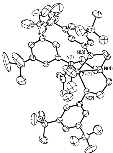
Fig. 2. Thermal ellipsoid plot of the molecular structure of [\text{Zr}(\text{TDT})(\text{CH}_2\text{Ph})] ( 8 ) (non-hydrogen atoms). Selected distances (Å) and angles (°): \text{Zr}(1)-\text{N}(2) 2.070(4), \text{Zr}(1)-\text{N}(3) 2.082(4), \text{Zr}(1)-\text{N}(1) 2.114(4), \text{Zr}(1)-\text{C}(49) 2.311(5), \text{Zr}(1)-\text{N}(4) 2.455(5), \text{N}(3)-\text{Zr}(1)-\text{N}(2) 117.23(18), \text{N}(3)-\text{Zr}(1)-\text{N}(1) 106.71(16), \text{N}(2)-\text{Zr}(1)-\text{N}(1) 111.05(17), \text{N}(3)-\text{Zr}(1)-\text{C}(49) 105.62(18), \text{N}(2)-\text{Zr}(1)-\text{C}(49) 102.36(18), \text{N}(1)-\text{Zr}(1)-\text{C}(49) 113.97(18), \text{N}(3)-\text{Zr}(1)-\text{N}(4) 71.87(15), \text{N}(2)-\text{Zr}(1)-\text{N}(4) 71.60(16), \text{N}(1)-\text{Zr}(1)-\text{N}(4) 75.43(15), \text{C}(49)-\text{Zr}(1)-\text{N}(4) 170.46(17).
