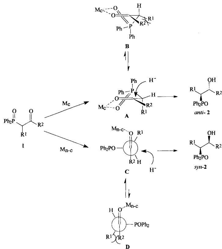
Scheme 1. Expected stereochemical control in the reduction of \alpha -alkyl- \beta -ketophosphine oxides with hydrides ( \text{H}^- ) in the presence of chelating ( \text{M}_\text{c} ) or nonchelating ( \text{M}_{\text{n-c}} ) Lewis acids.
