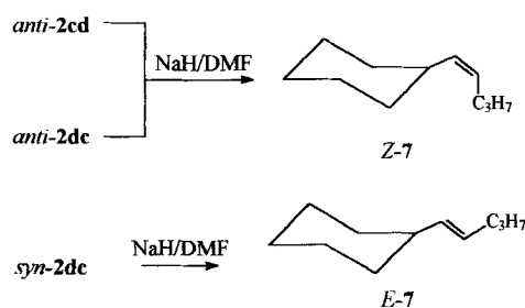
Scheme 9. Synthesis of ( Z )- and ( E )-1-cyclohexyl-1-pentene.
