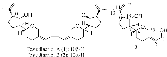
Figure 1. Structures of testudinariol A, B and the key intermediate.
